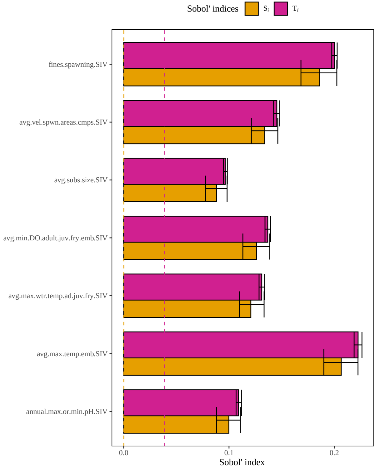
Figure 5. Results of a sensitivity analysis for the cutthroatLacGenMt15C model based on a geometric mean structure. Dashed lines represent baseline numerical approximation error for S_i and T_i ( i.e. , dummy variables).
